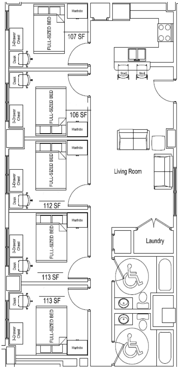
Sample floor plan #3 5 Bedroom Suite
